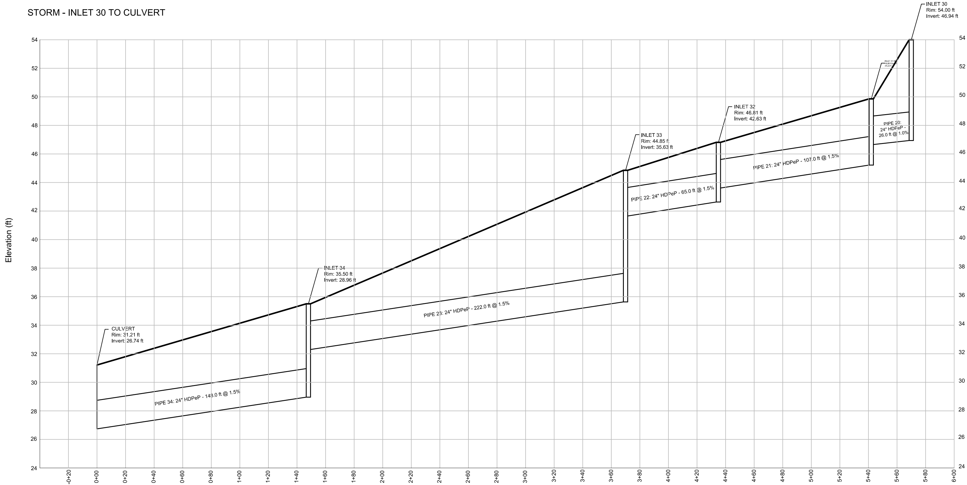
STORM - INLET 30 TO CULVERT
