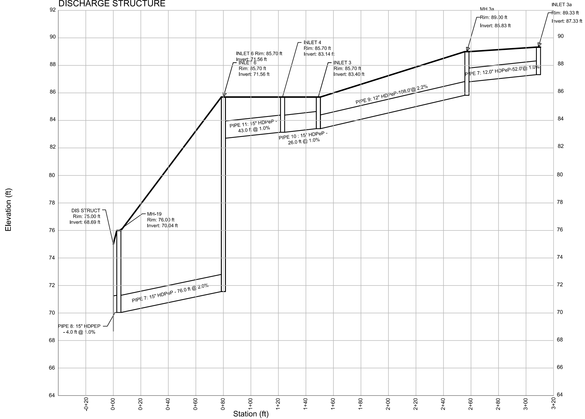
STORM - INLET 3a TO DISCHARGE STRUCTURE
