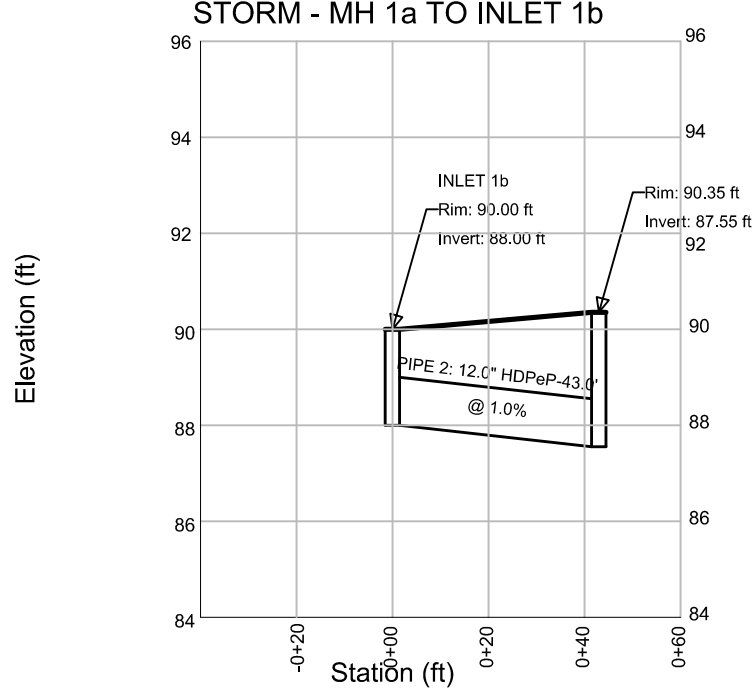
STORM - MH 1a TO INLET 1b
